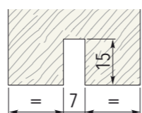
7 mm - Frezarea standard fara profil security
